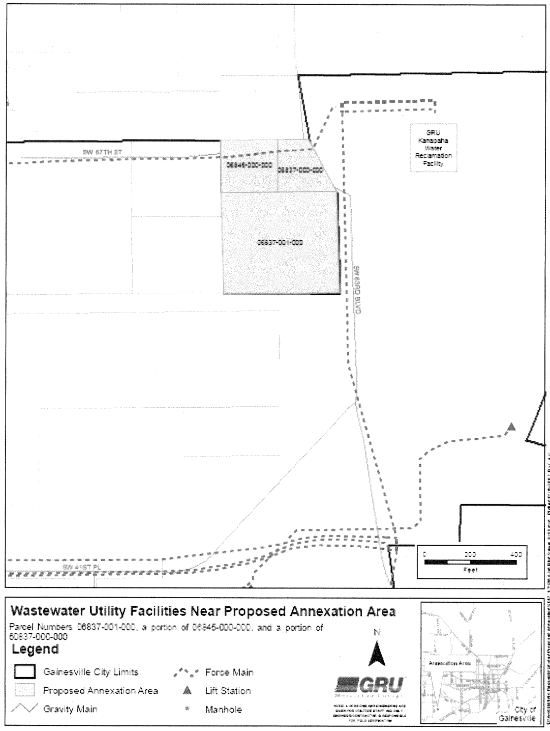
Figure 5: Wastewater Utility Facilities
