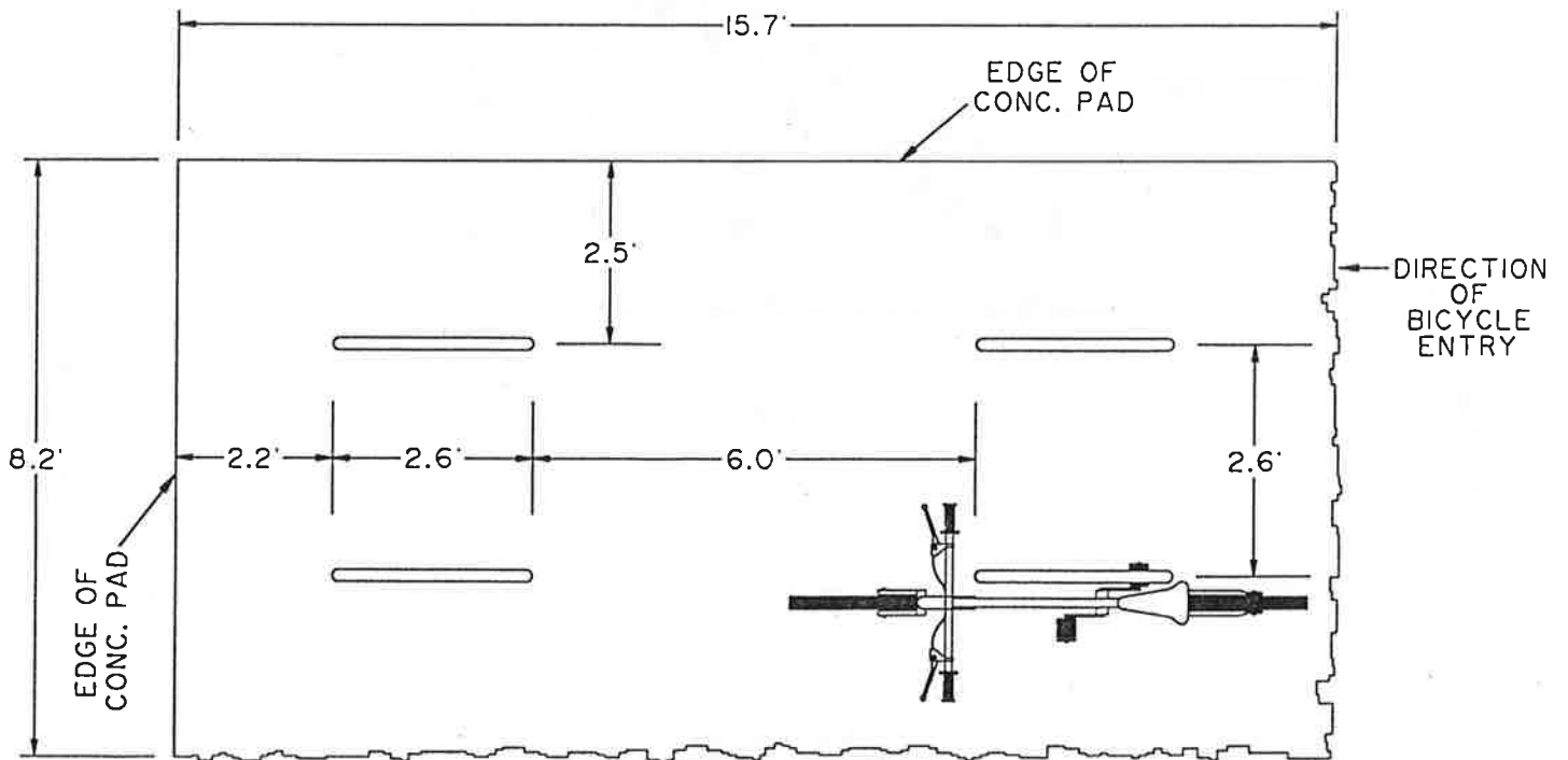
PLAN VIEW
