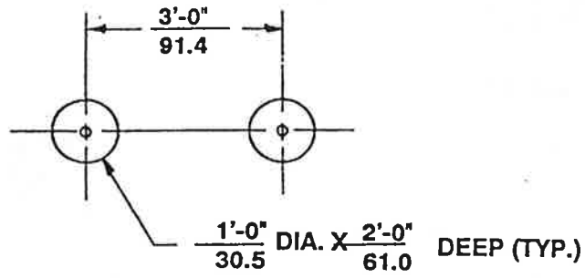
7703 GROUND PLAN
