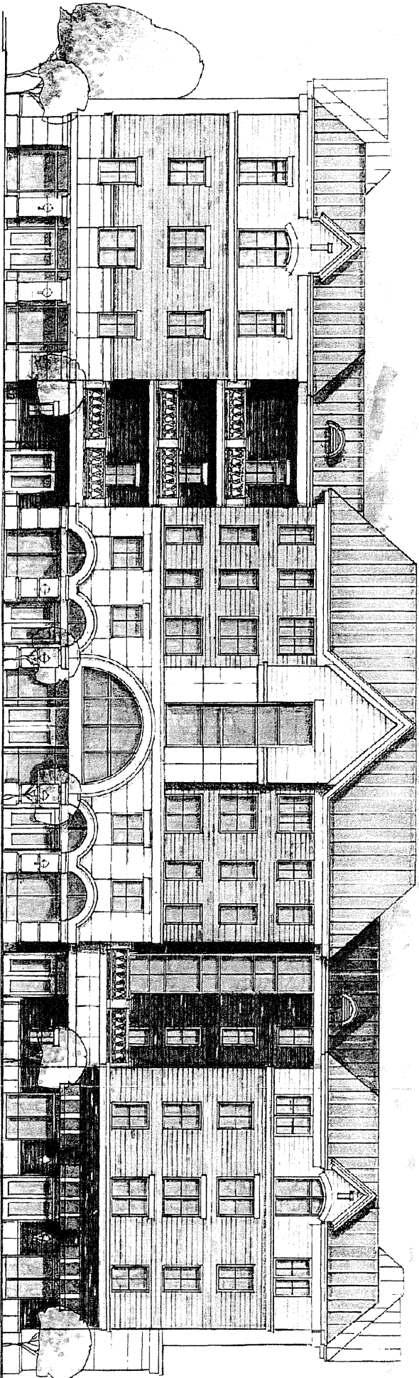
southwest first avenue elevation
