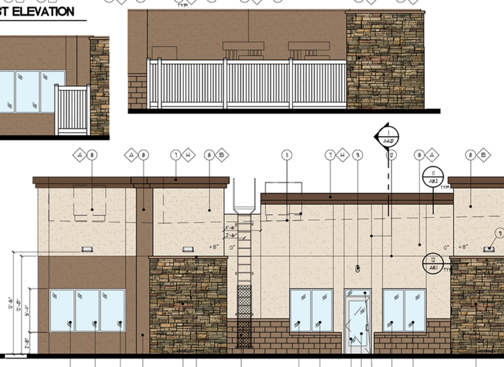
4 SOUTHWEST ELEVATION SCALE: 3/16" = 1'-0"
