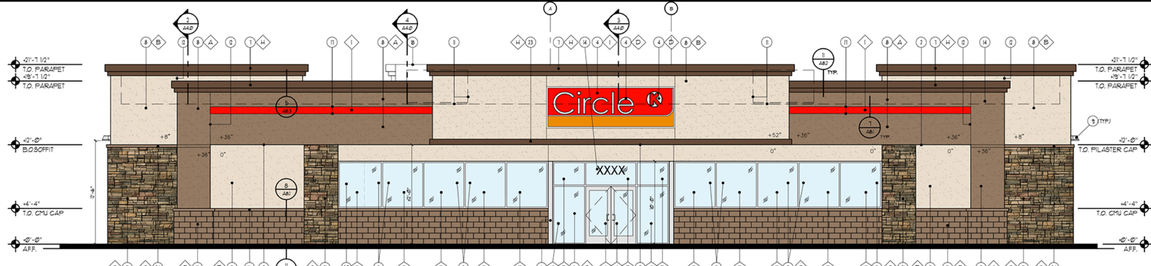
1 SOUTHEAST ELEVATION SCALE: 3/16" = 1'-0"
