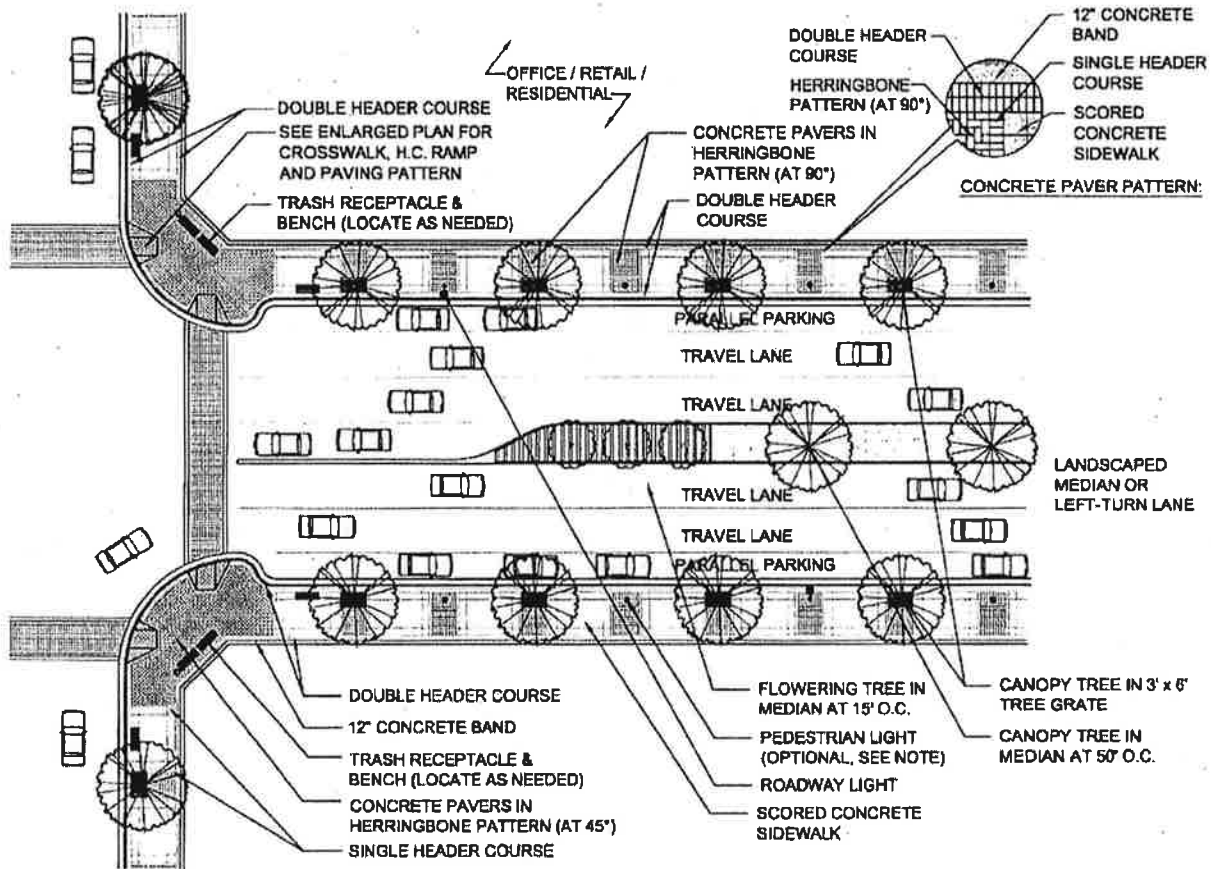
TYPICAL PLAN WITH PARALLEL PARKING
