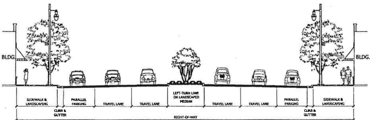
ROADWAY SECTION WITH PARALLEL PARKING
