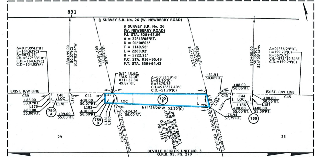
DETAIL No. 6 FROM SHEETS 11 & 12 NOT TO SCALE
