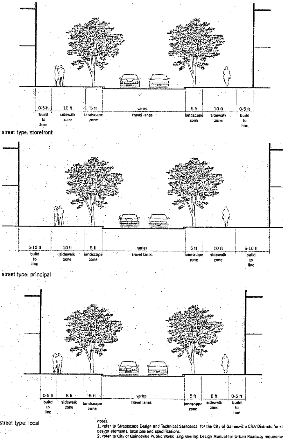
Fig. 2.4 - District Framework Plan - Public Realm Requirements
