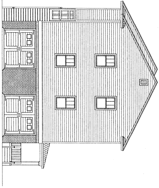
MODIFIED GARAGE BUILDING NORTH ELEVATION BEHIND 1101 S.W. 5TH AVENUE
