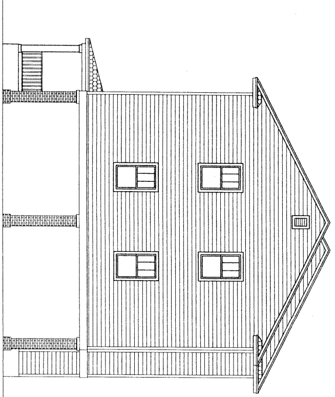
MODIFIED GARAGE BUILDING SOUTH ELEVATION BEHIND 1101 S.W. 5TH AVENUE
