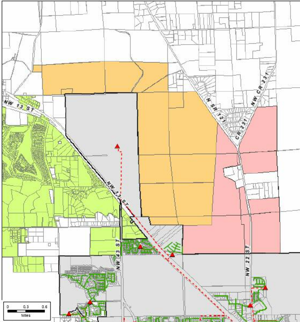
Figure 5: Wastewater Utility Facilities
