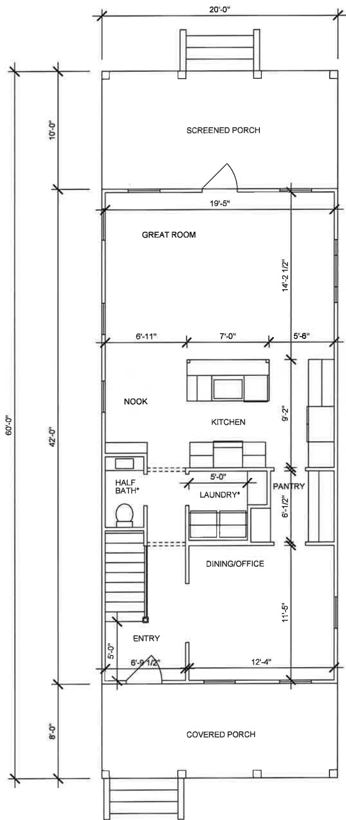
FIRST FLOOR FLOOR PLAN
